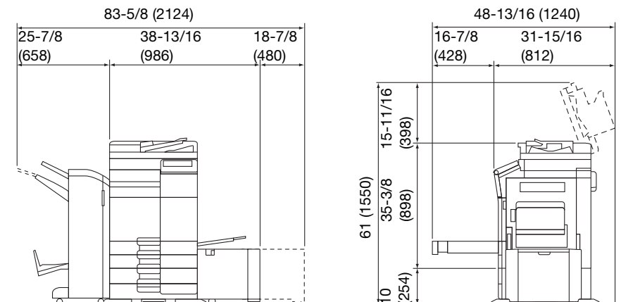
bizhub C368/C308/C258 + DF-629 + PC-210 + FS-534 + SD-511 + RU-513 + LU-302 Μονάδα: ίντσα (mm)
