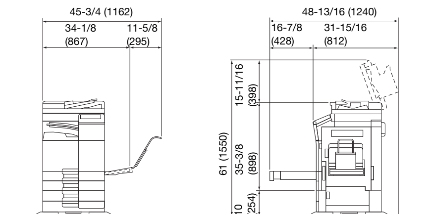
bizhub C368/C308/C258 + DF-629 + PC-210 + JS-506 + MK-730
