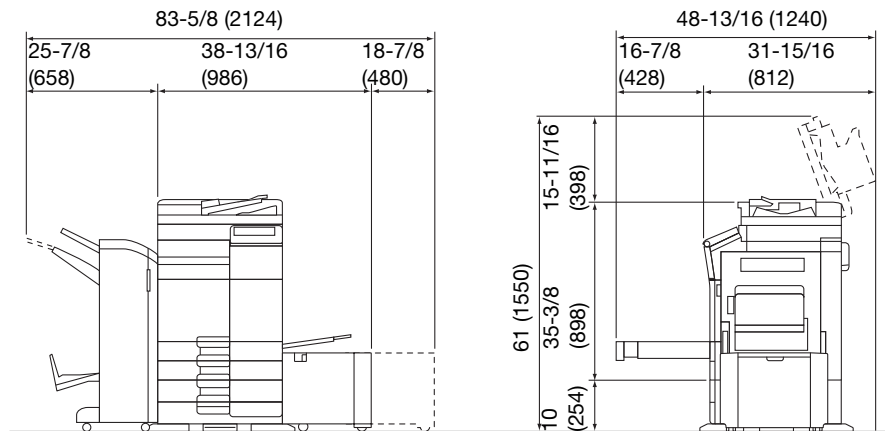
bizhub C368/C308/C258 + DF-629 + PC-210 + FS-534 + SD-511 + RU-513 + LU-302
